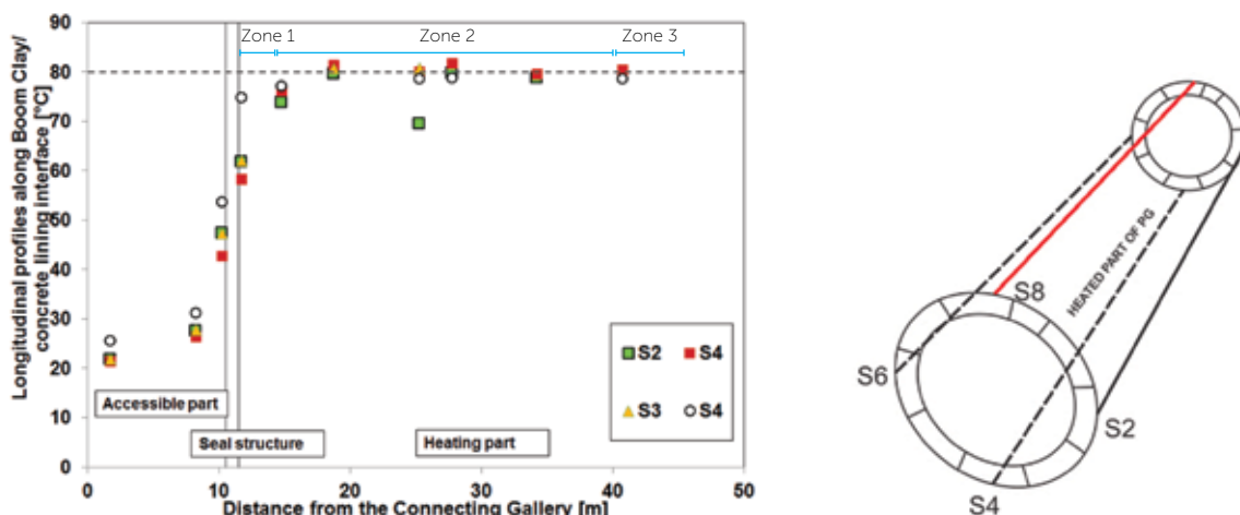
Figure 10 - Longitudinal profiles of the temperature along the extrados of the PRACLAY gallery (end 2016)
