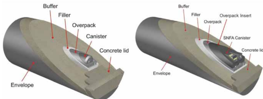
Figure 30 - Supercontainer layout
