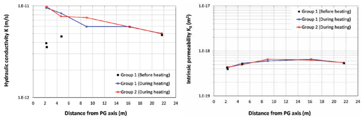
Figure 24 - Hydraulic conductivity (left) and intrinsic permeability (right) measured on the two groups of filters before and during heating
