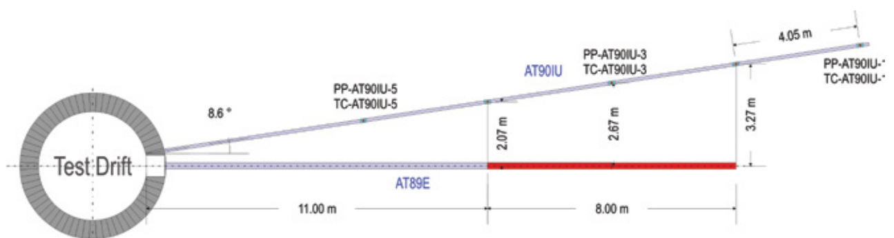
Figure 19 - Upward borehole AT90IU drilled above the heater for ATLAS IV
