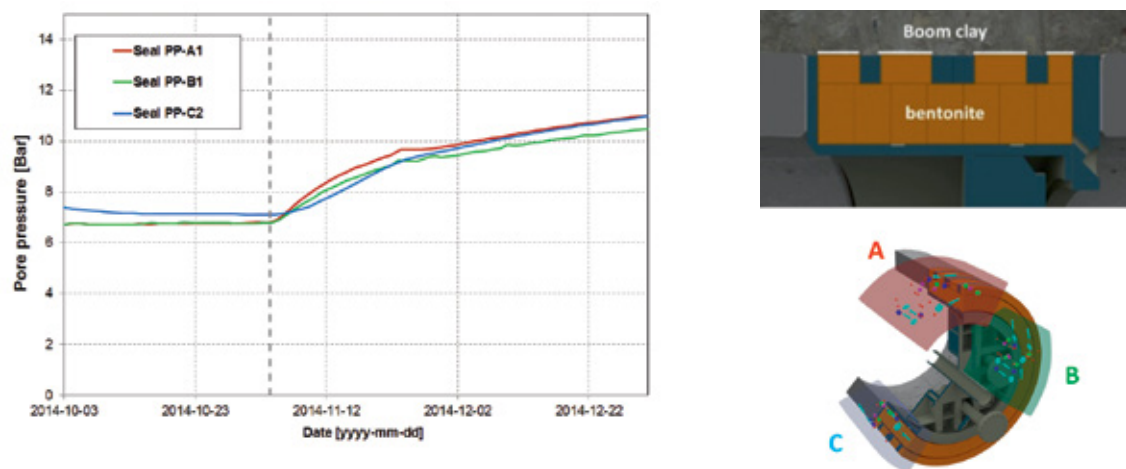
Figure 9 - Pore water pressure at the interface between the bentonite and the Boom Clay (white line in insert), for sections A, B and C
